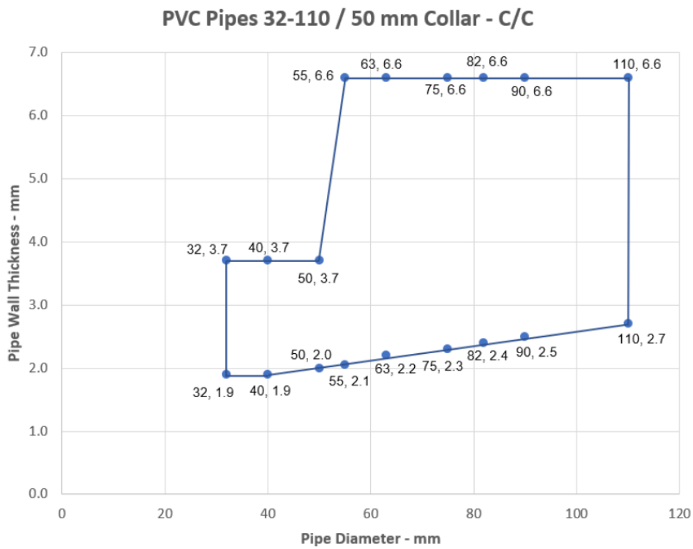
Figure 41 Intermediate pipe wall thicknesses for PVC pipe diameters 32 mm – 110 mm
