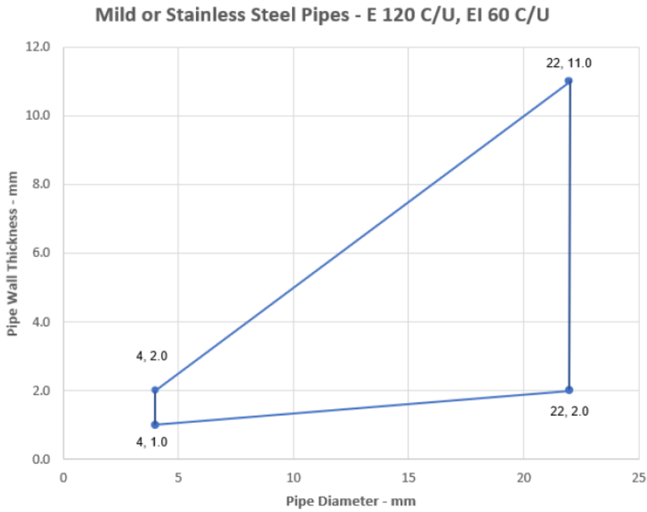
Figure 19 Intermediate pipe wall thicknesses for mild or stainless steel pipe diameters
