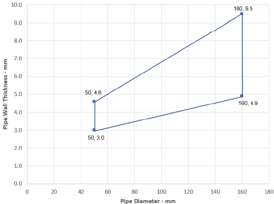
Figure 27 Intermediate pipe wall thicknesses for PE pipe diameters
