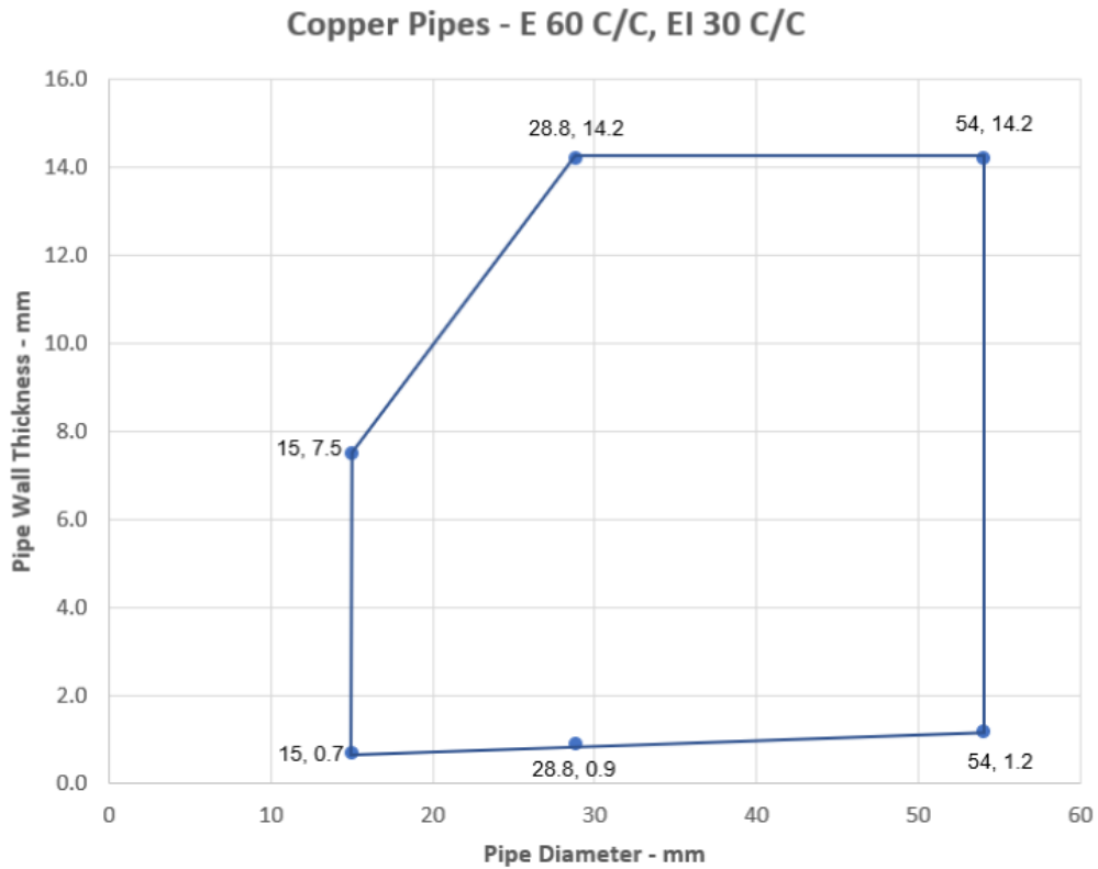
Figure 38 Intermediate pipe wall thicknesses for copper pipe diameters with CS insulation
