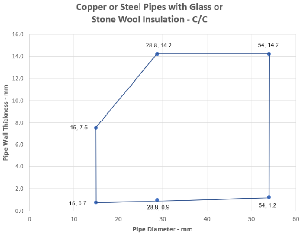
Figure 20 Intermediate pipe wall thicknesses for copper or steel pipe diameters with Glass or Stone wool insulation. Applicable to C/C end conditions.
