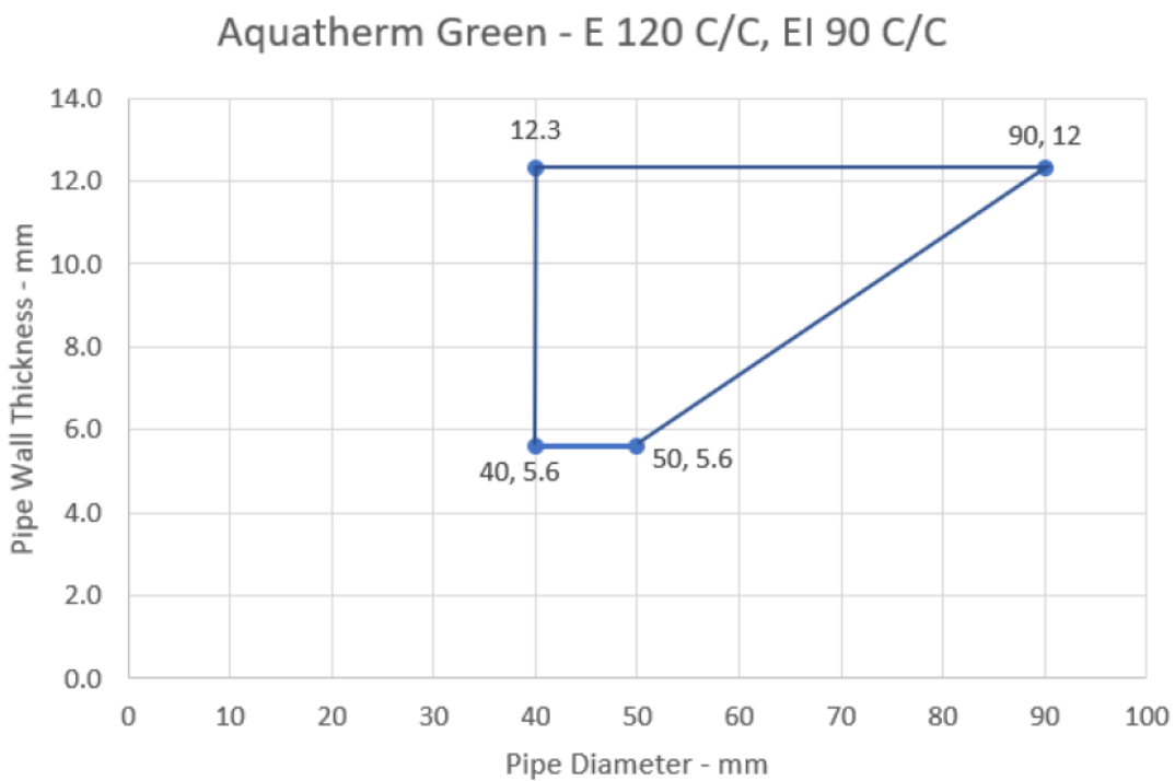
Figure 33 Intermediate pipe wall thicknesses for Aquatherm Green pipe diameters
