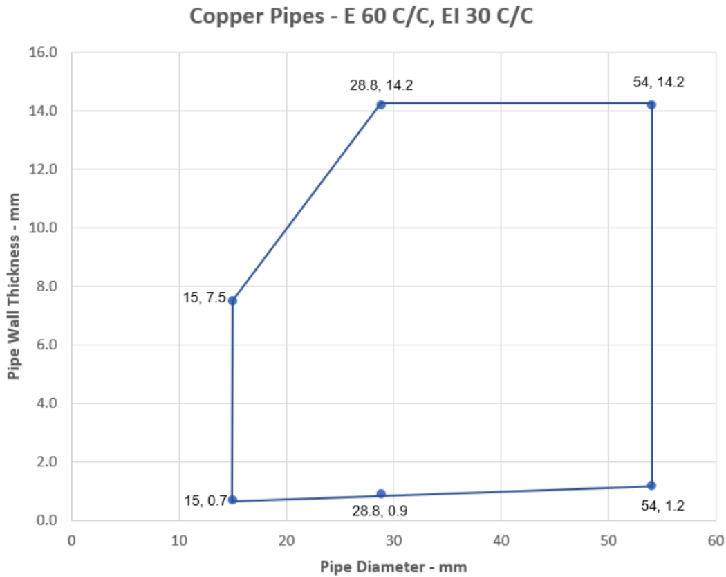
Figure 40 Intermediate pipe wall thicknesses for copper pipe diameters with CS insulation
