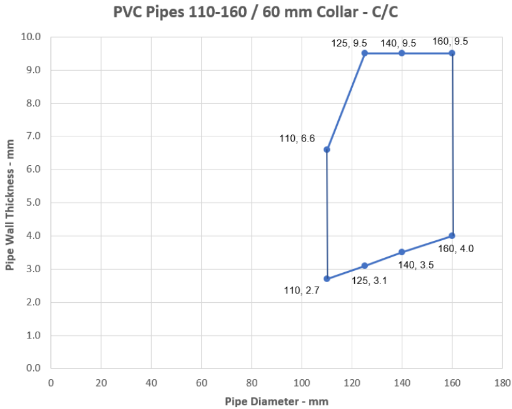
Figure 42 Intermediate pipe wall thicknesses for PVC pipe diameters 110 mm – 160 mm
