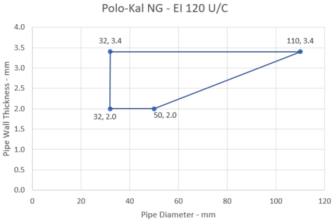
Figure 32 Intermediate pipe wall thicknesses for Polo-Kal NG pipe diameters
