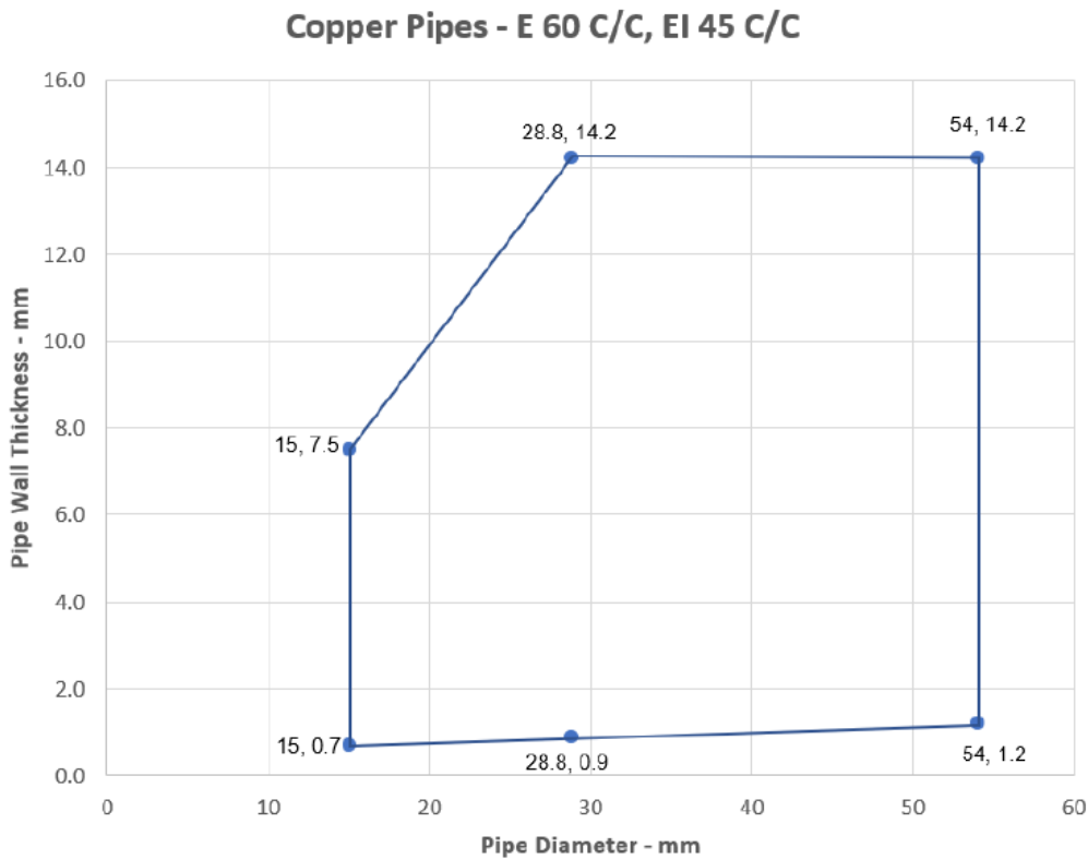
Figure 39 Intermediate pipe wall thicknesses for copper pipe diameters with CI insulation
