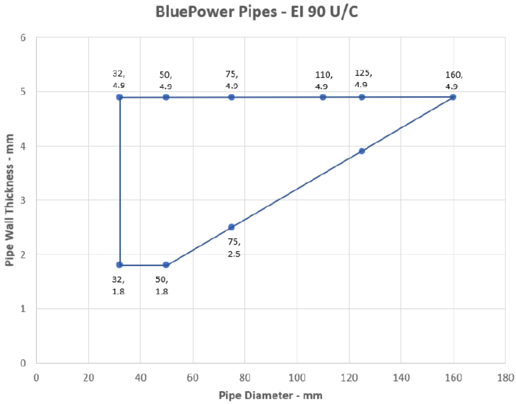
Figure 30 Intermediate pipe wall thicknesses for BluePower pipe diameters
