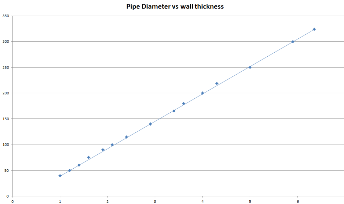
Figure 23 Intermediate pipe wall thicknesses for mild or stainless steel pipe diameters
