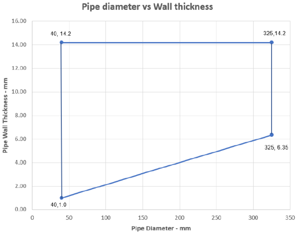
Figure 10 For 75 mm thick walls, intermediate pipe wall thicknesses for typical mild or stainless steel pipe diameters - 50 mm stone wool min. 80 kg/m 3
