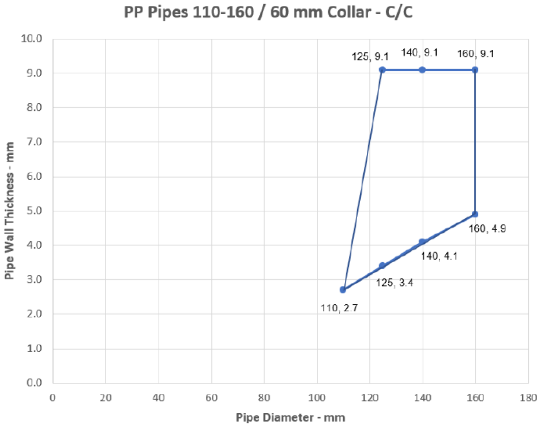
Figure 46 Intermediate pipe wall thicknesses for PP pipe diameters 110 mm – 160 mm
