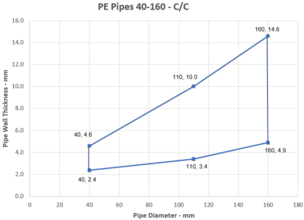
Figure 48 Intermediate pipe wall thicknesses for PE pipe diameters 40 mm – 160 mm
